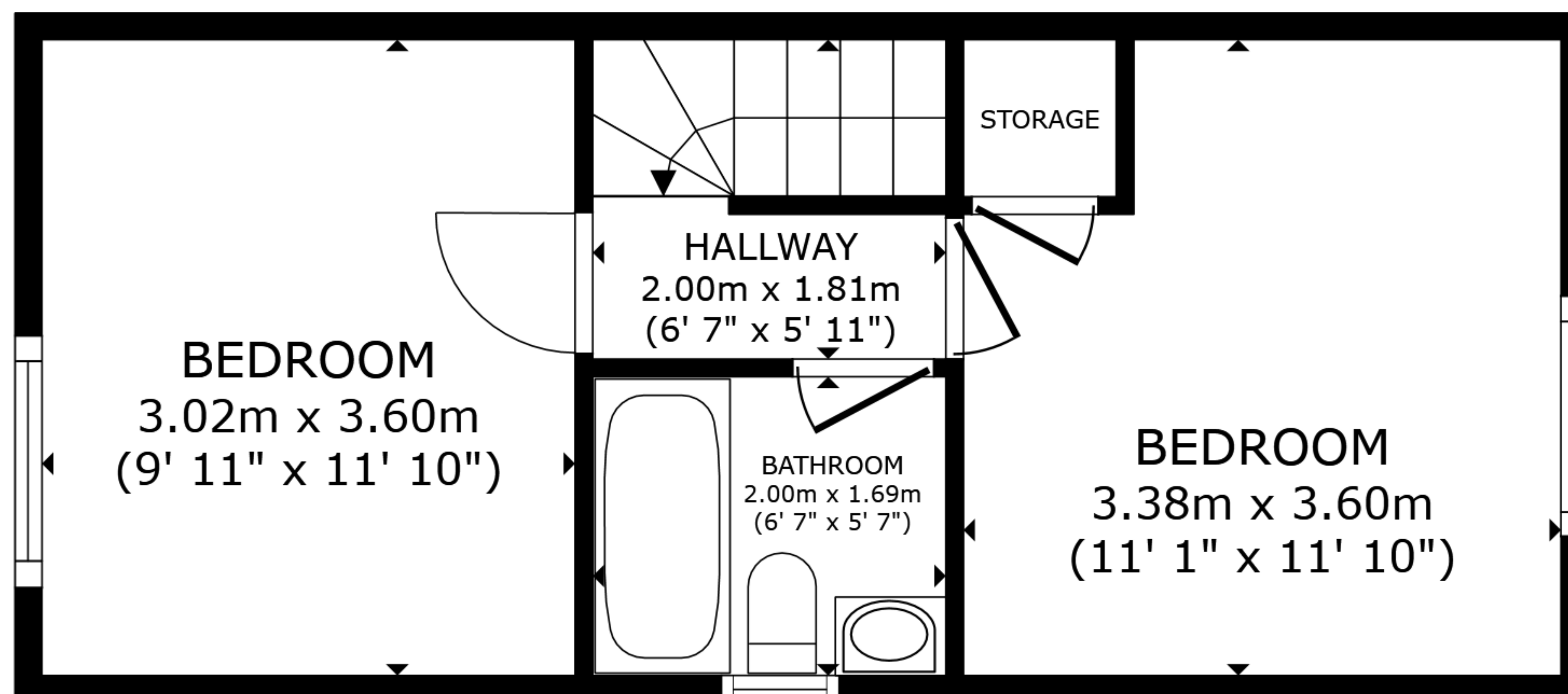
FLOOR 2
