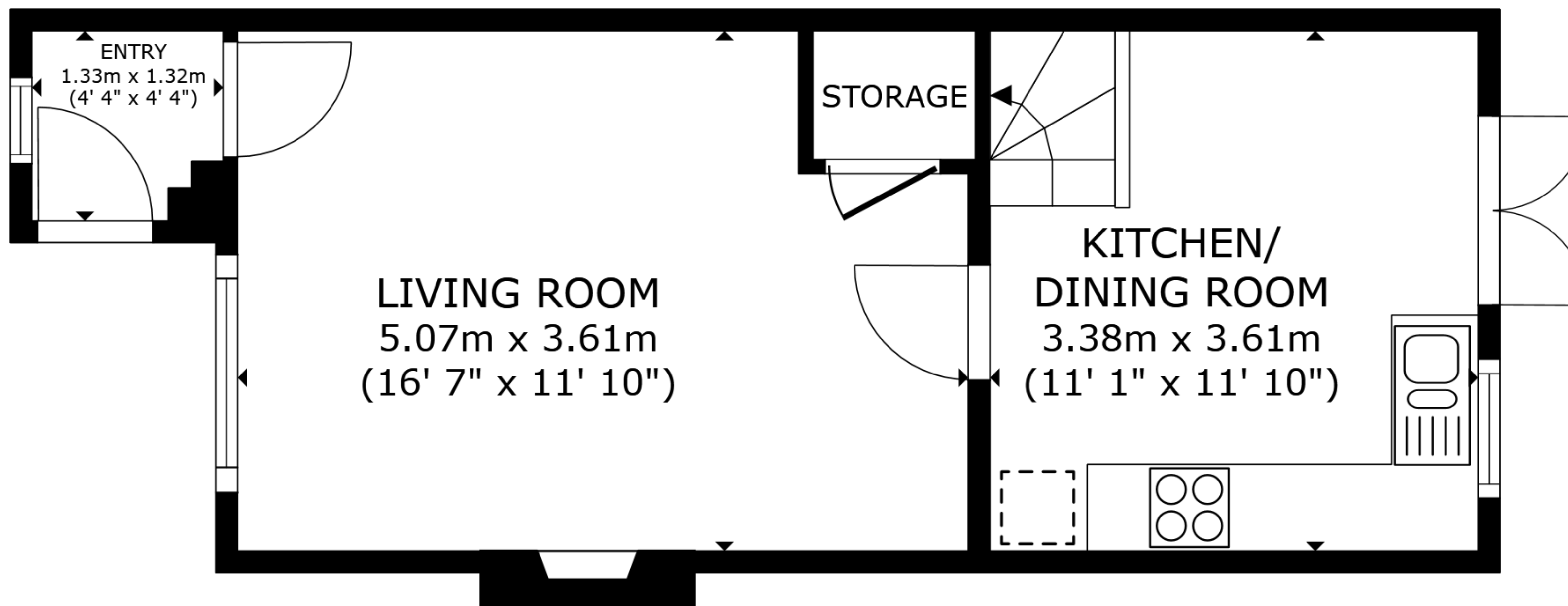
FLOOR 1
